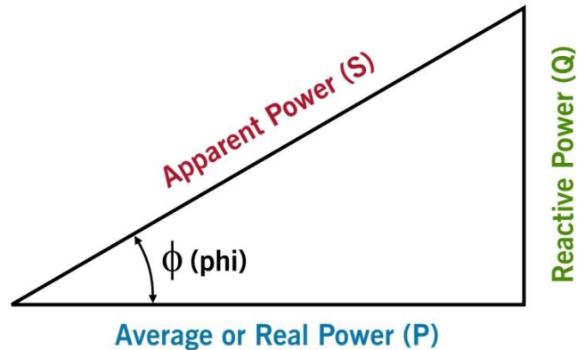
Figure A-2. Power Triangle
