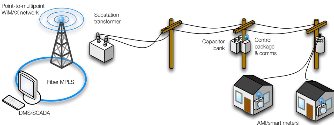
Figure 10. PPL's VVO Configuration
